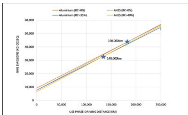
Figure 3: Cumulative lifecycle emissions (by distance driven) for a family car (gasoline internal combustion engine) with an aluminum and AHSS BIW incorporating a range of recycled contents (RC). The distance at which a family car with an aluminum BIW begins to save lifetime GHG emissions compared to an AHSS vehicle (at a recycled content of 0%/0% and 35%/40%) are indicated by a star.
