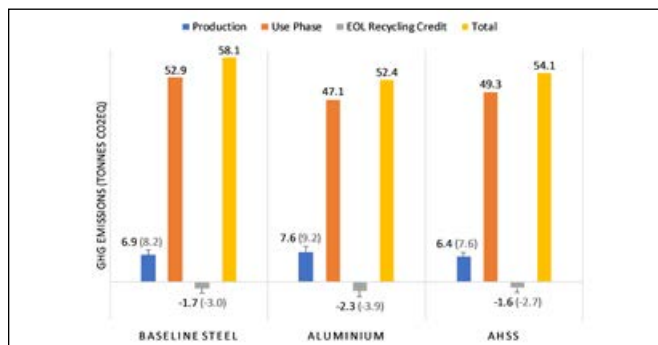
Figure 2: Lifecycle CO 2 e emissions by stage comparing a mild steel, aluminum, and AHSS BIW for a family car with a gasoline internal combustion engine. Error bars and values in brackets represent the results with zero percent recycled metal content.
