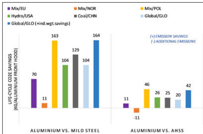
Figure 4: Total lifecycle CO 2 e savings for an aluminum front hood used in a battery electric vehicle taxi compared to a mild steel or an AHSS front hood. A 35% indirect weight savings can be applied to visualize GHG savings from downsizing of the vehicle components.
