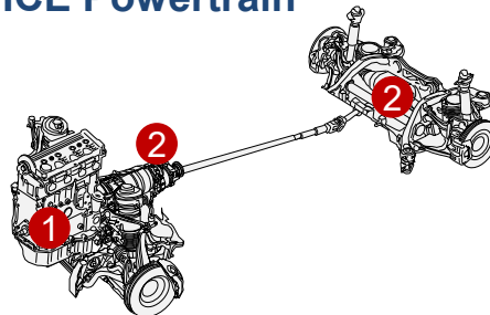
ICE Powertrain
