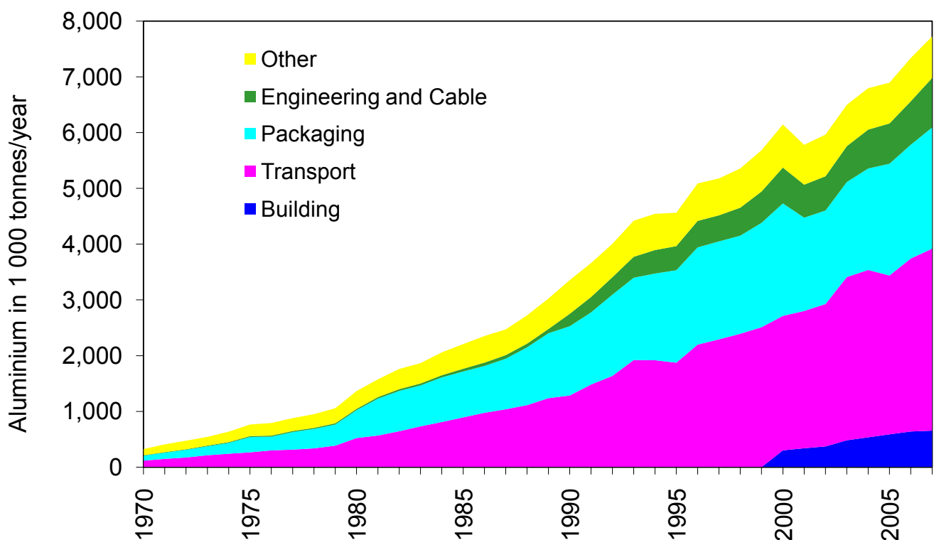
Figure 15: Global Old Scrap Recycled by Market
