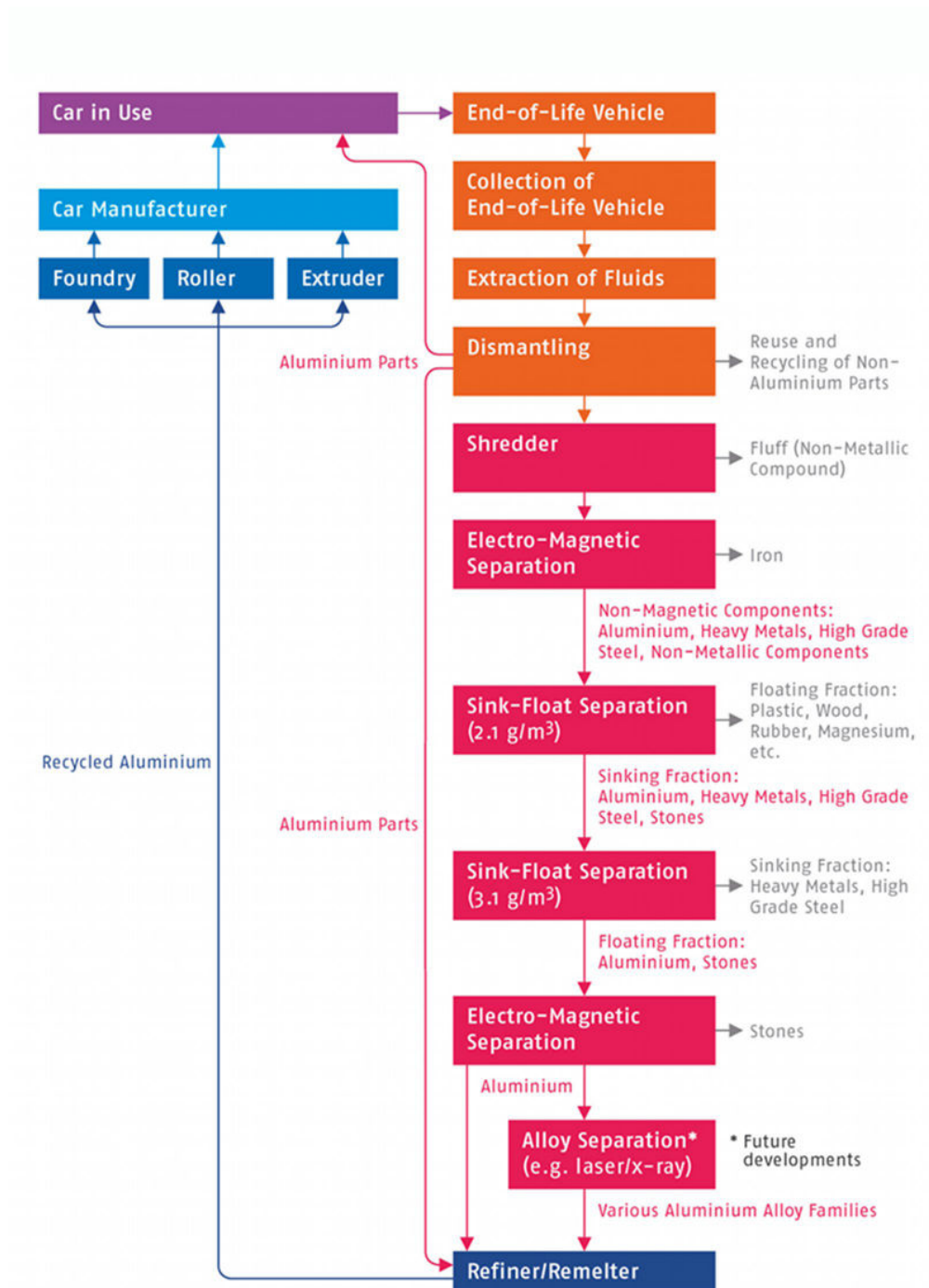
Figure 10: Modern End-of-Life Vehicle Dismantling and Aluminium Recycling Process
