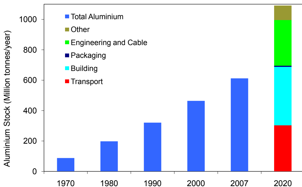
Figure 18: Build-up of Aluminium in Use by 2020
