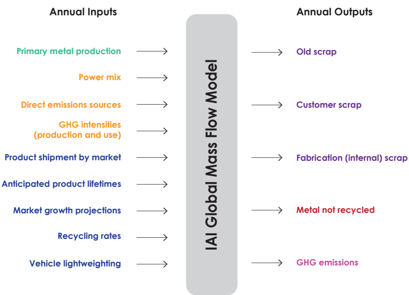
Fig 5.9 Inputs and outputs annually for the IAI Global Mass Flow Model
